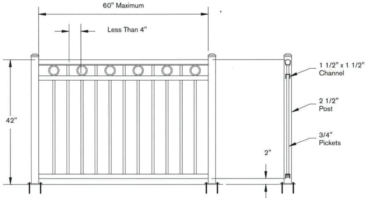
STAGGERED PICKETS WITH RING DESIGN
