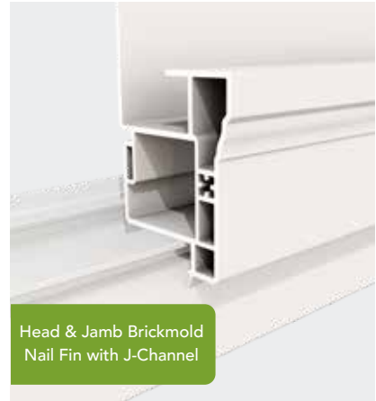
Brickmold with 3/4" J-Channel with Nail Fin (Also available with 1 1/8" J-Channel with Nail Fin)
